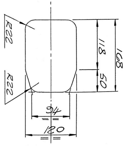
CORE DETAIL.
